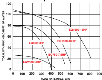
EQ Series performance curve
